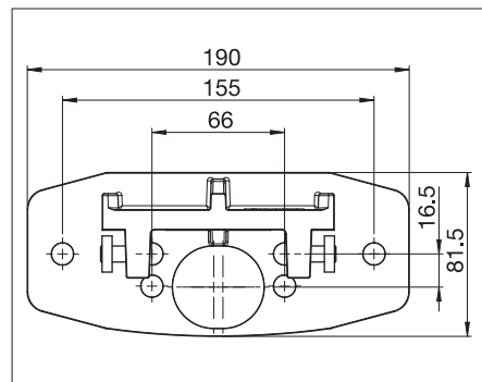
P809/5 Fotplatta
