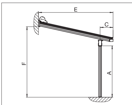
GP5200 E = max. 500 cm/C=100 cm/E-C = max. 400 cm
