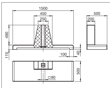
OS617 Betongsockel (ca 186 kg)
