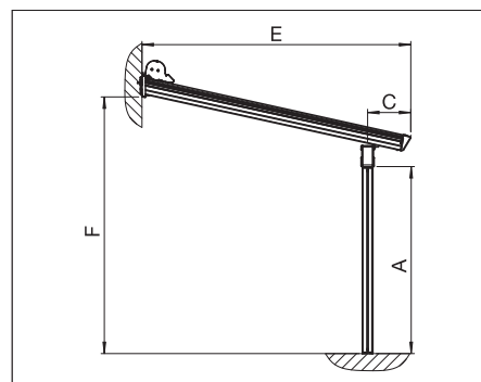
GP5300 E = max. 500 cm/C = 23-100 cm/E-C = max. 400 cm
