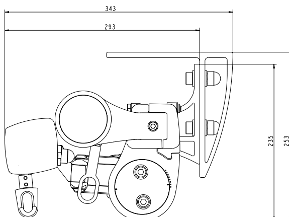
FA44 with Roller Valance
