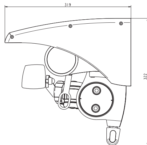
FA44 with Roller Valance & Hood
