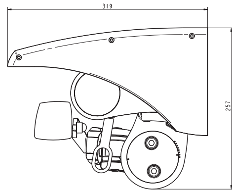
FA44 with Pitch Control & Hood
