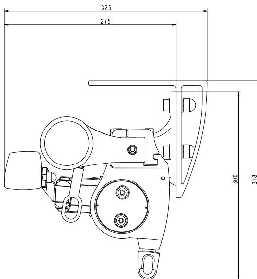
FA44 with Roller Valance
