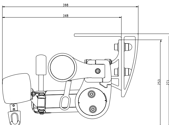
FA46 with Roller Valance
